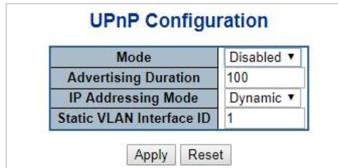
Figure 4-2-1-10-1: UPnP Configuration Page Screenshot
