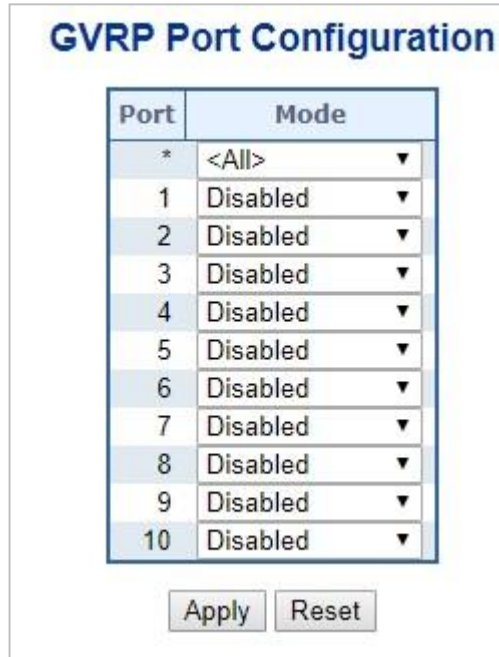
Figure 4-3-8-2: GVRP Port Configuration Page Screenshot
