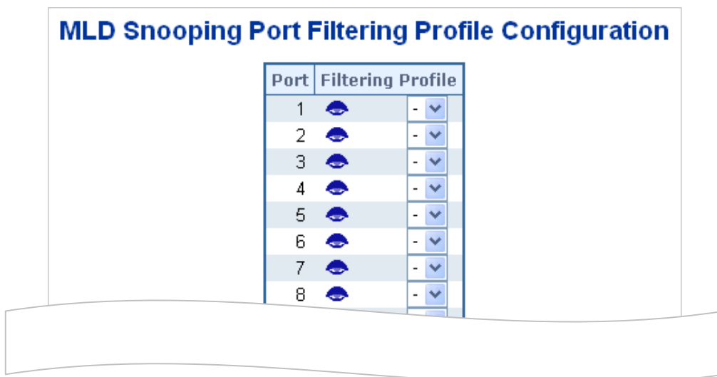
Figure 4-3-12-3: MLD Snooping Port Group Filtering Configuration Page Screenshot
