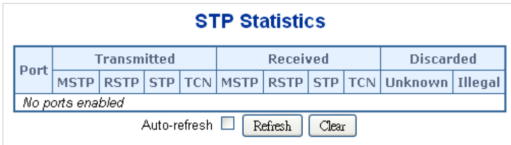
Figure 4-3-10-9: STP Statistics Page Screenshot
