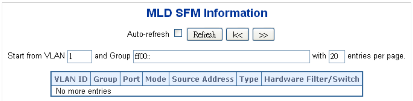
Figure 4-3-12-6: MLD SSM Information Page Screenshot
