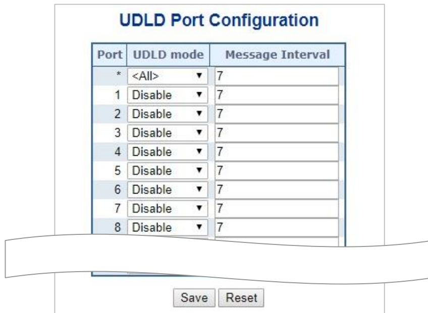
Figure 4-3-17-1: UDLD Configuration Page Screenshot
