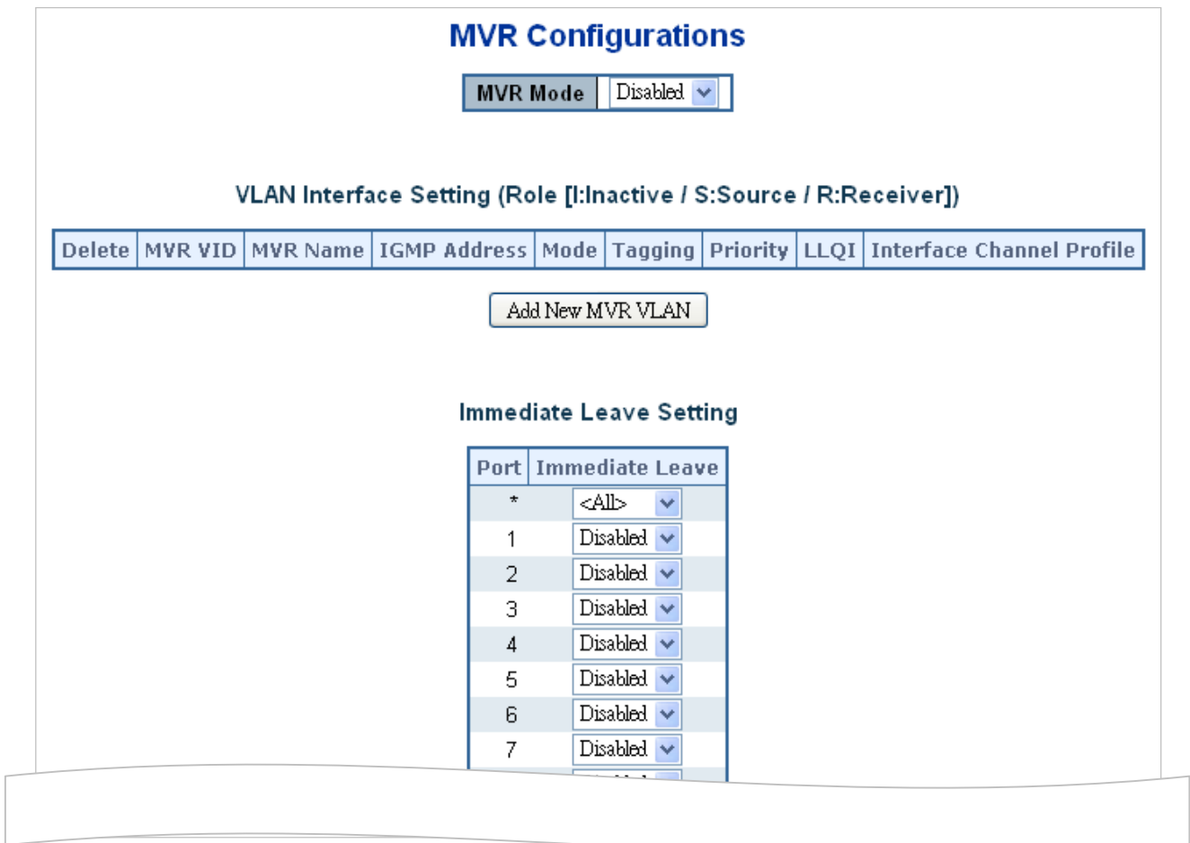
Figure 4-3-13-1: MVR Configuration Page Screenshot
