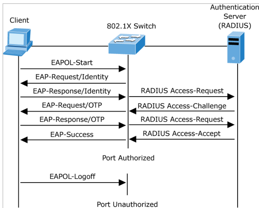
Figure 4-6-2-2: EAP Message Exchange
