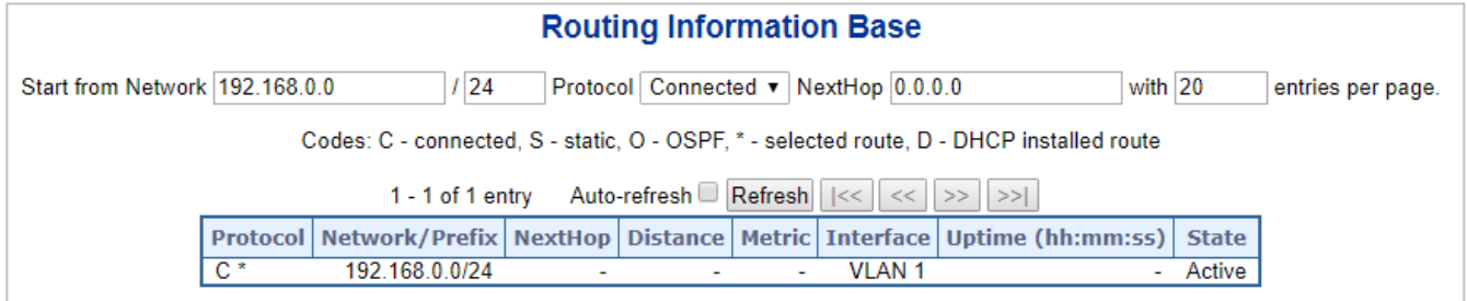
Figure 4-4-3: IP Status Page Screenshot
