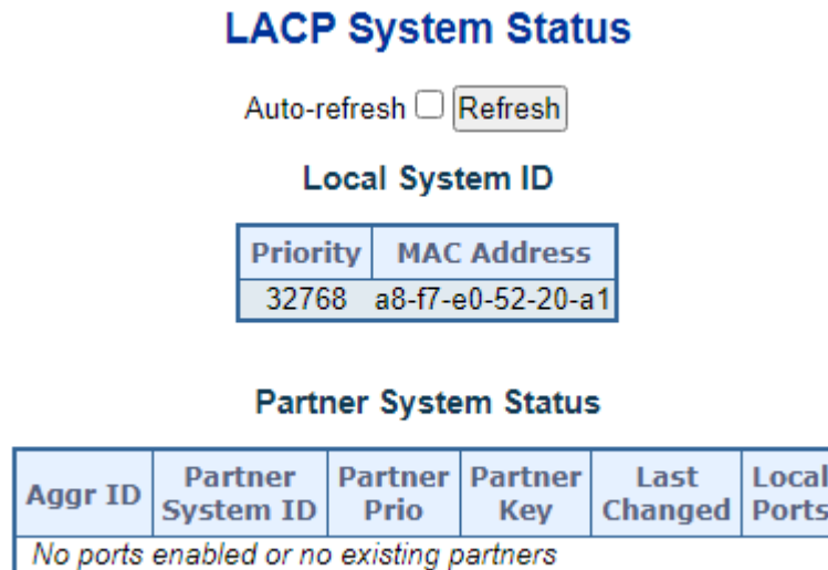
Figure 4-3-2.5: LACP System Status Page Screenshot
