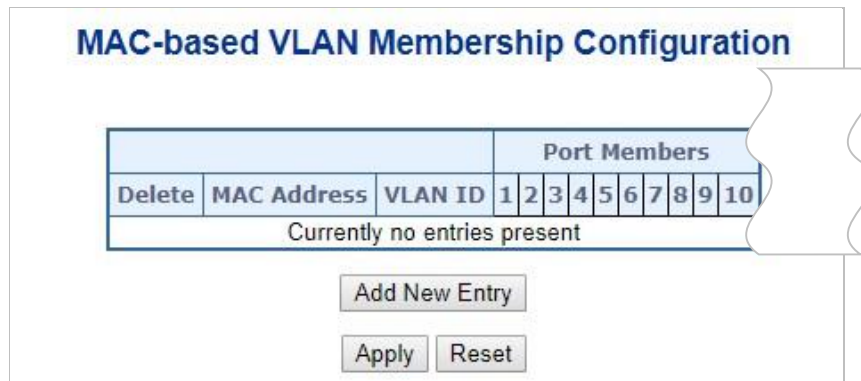
Figure 4-3-7-1: MAC-based VLAN Membership Configuration Page Screenshot
