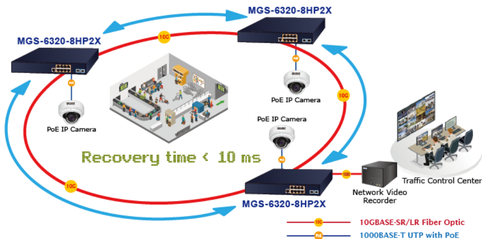
Figure 4-7-1-2: Ring Example Diagram
