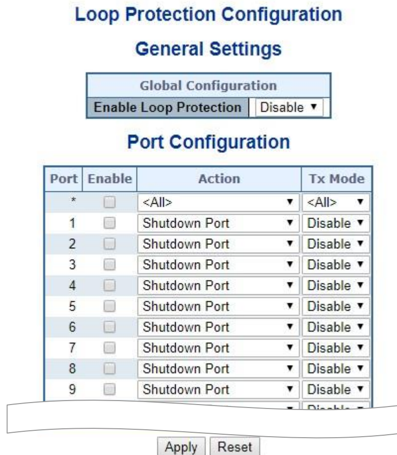
Figure 4-3-16-1: Loop Protection Configuration Page Screenshot
