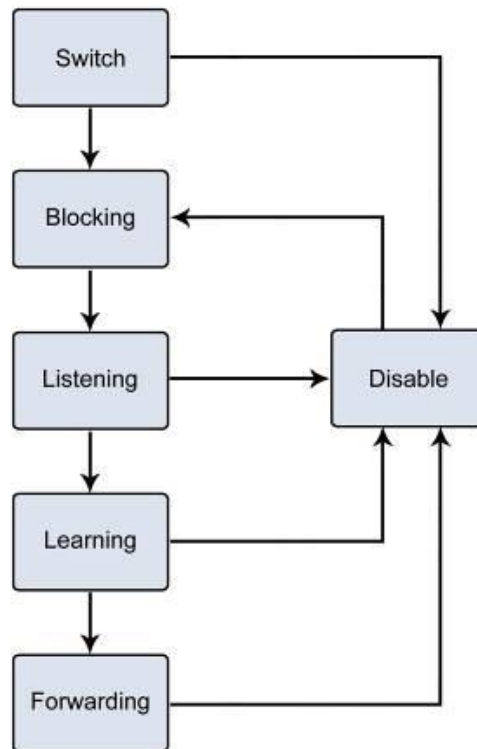
Figure 4-3-10-1-1: STP Port State Transitions
